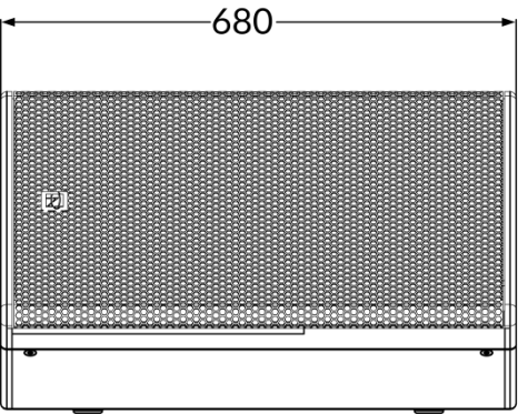
Dimensional Drawing (mm)
