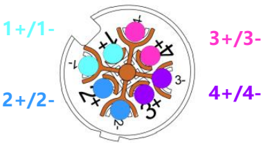
Output Connector
