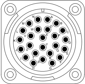
Female Connector
