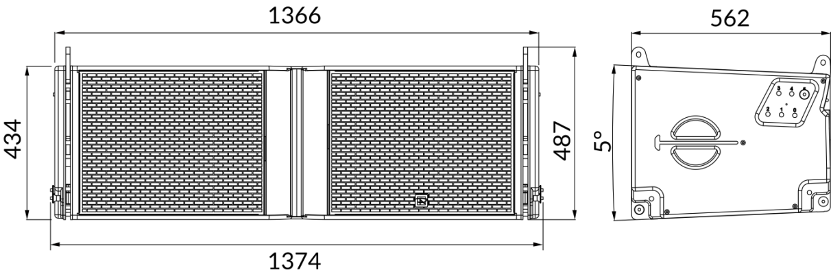
Dimensional Drawing (mm)
